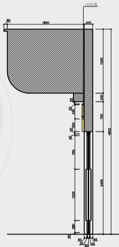
剖面图-1
